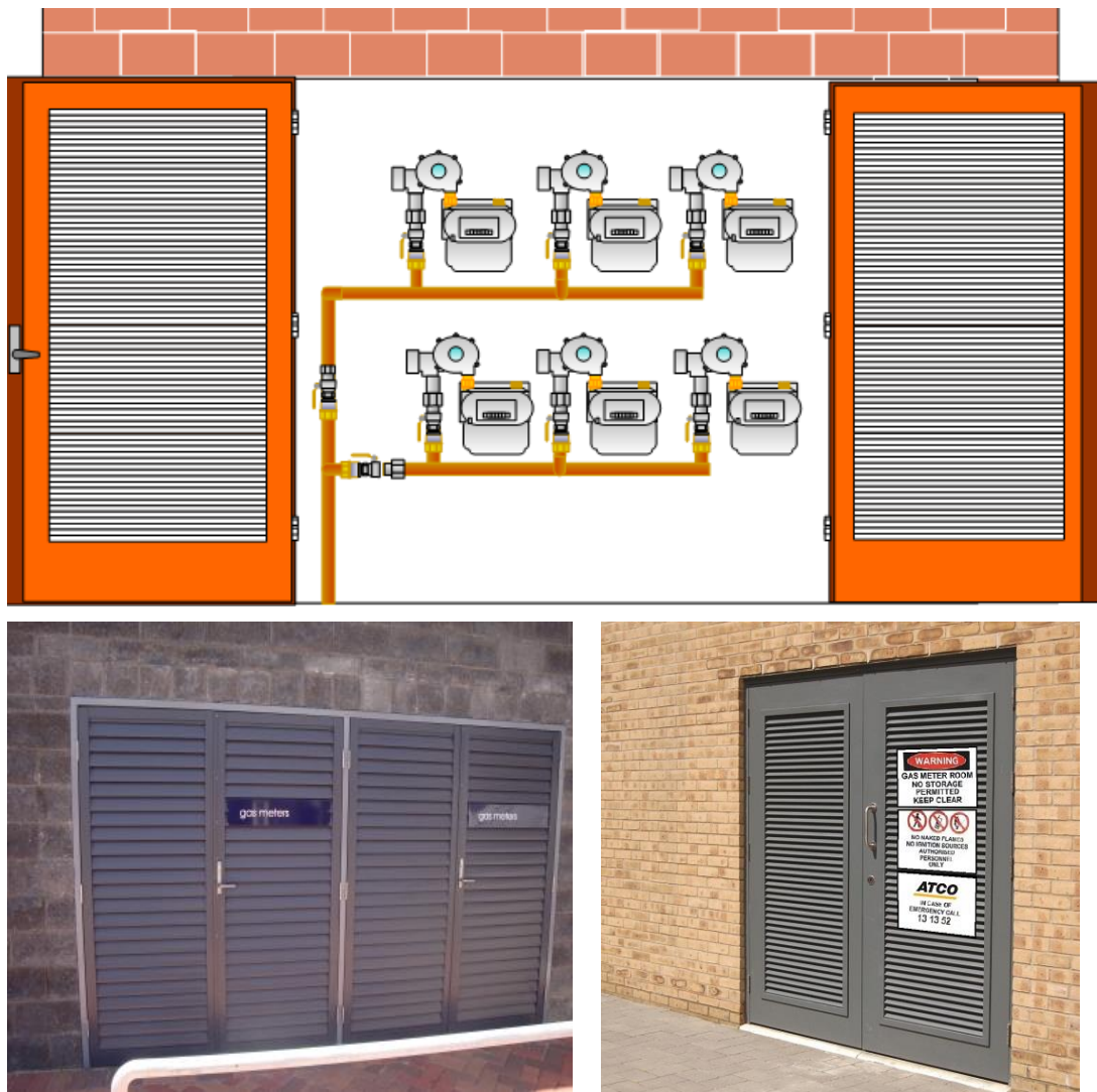
Figure 56: Recess or Enclosure with Fully Louvered Doors (Examples)
